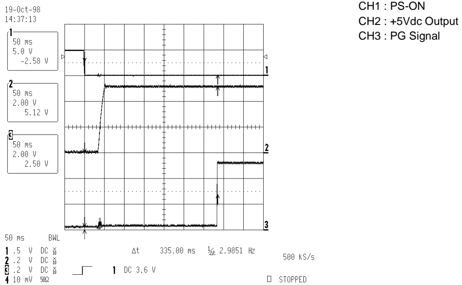
Figure 4. PG Signal Delay Time
