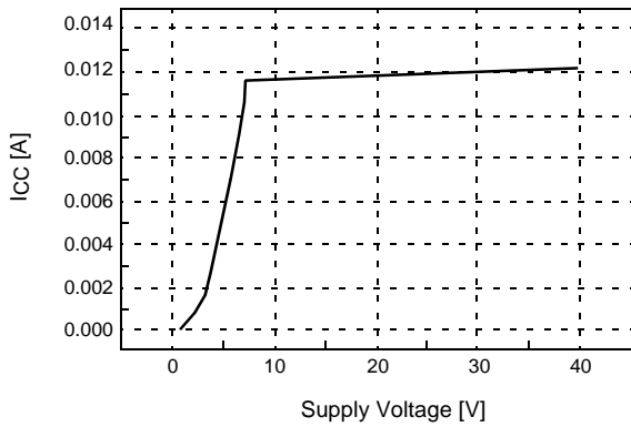
Figure 1. V CC -I CC
