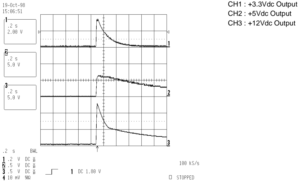
Figure 6. No Load Protection
