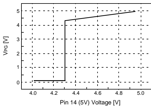
Figure 15. Detecting V5 Voltage
