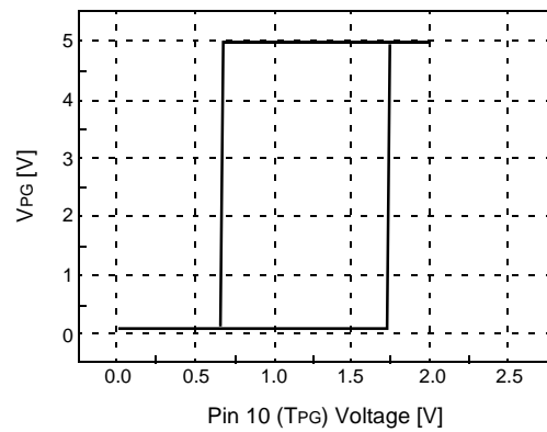
Figure 16. Hysteresis Voltage 2
