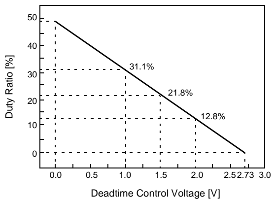
Figure 3. PIN19(Dead Time Control Voltage)-Duty Cycle
