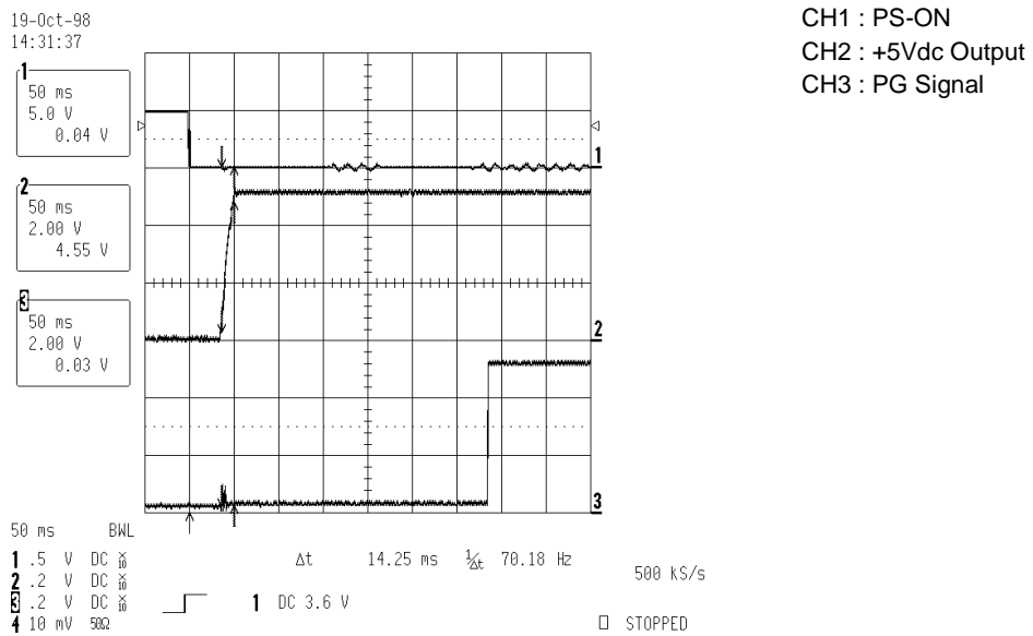
Figure 3. Rising Time of +5Vdc Output Voltage
