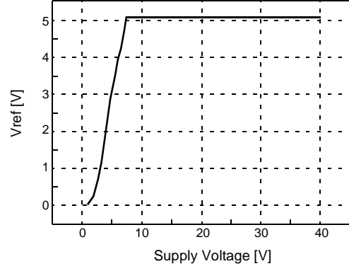
Figure 18. Reference Voltage
